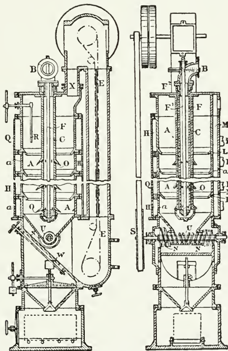
Fig. 84—Decomposer, Mond Refining Process.
